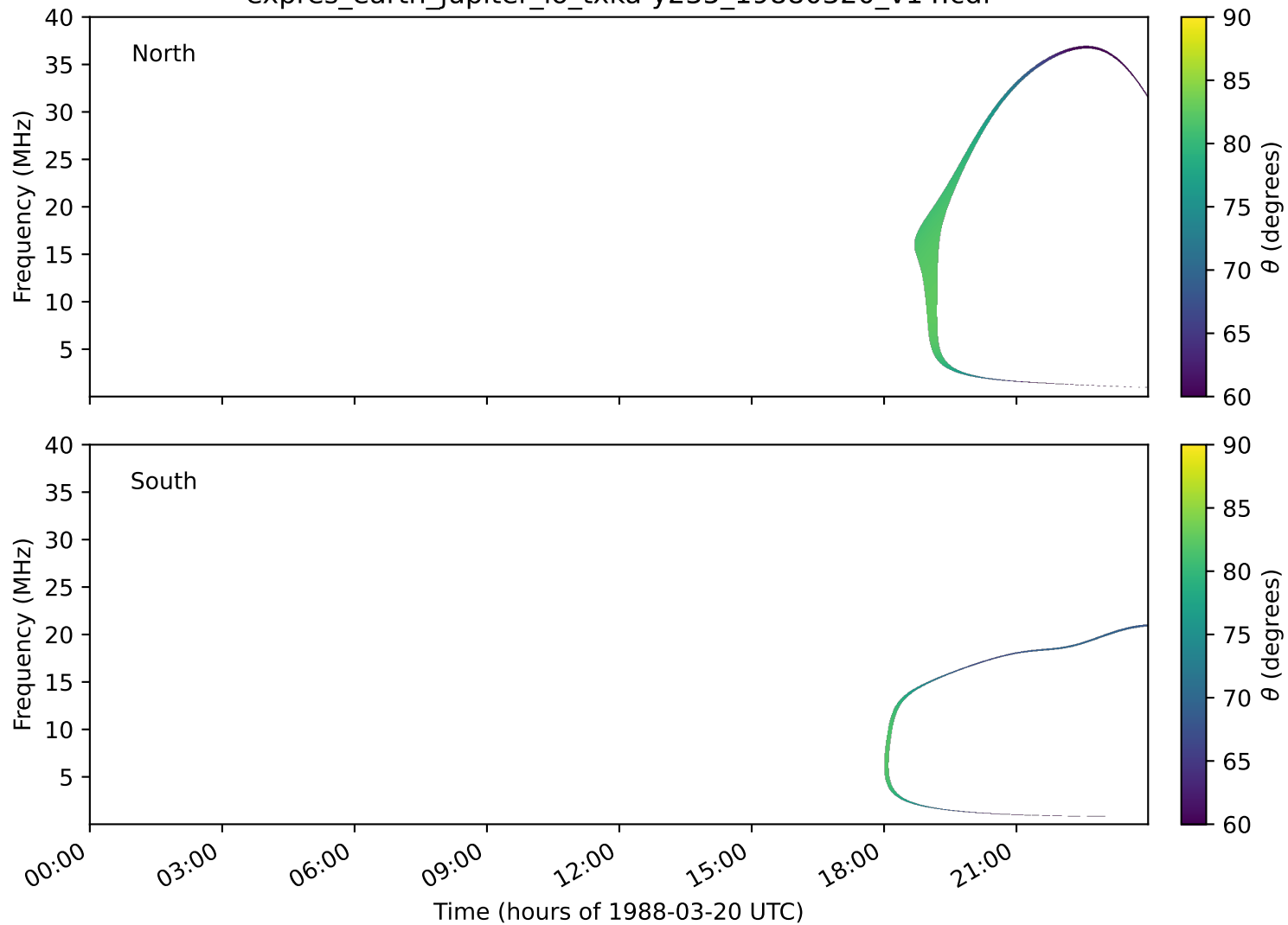
expres_earth_jupiter_io_txka-y235_19880320_v14.cdf
