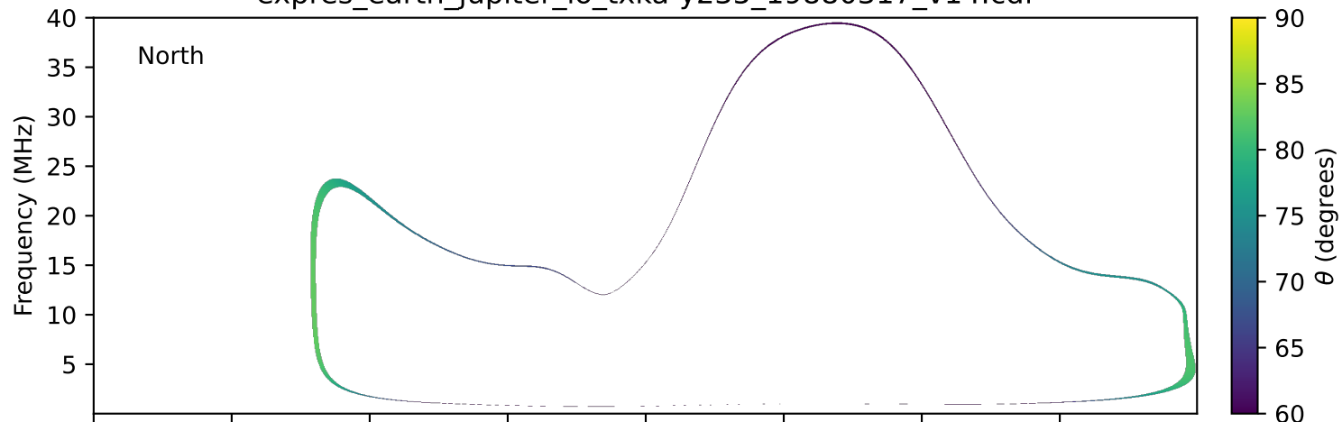
expres_earth_jupiter_io_txka-y235_19880317_v14.cdf
