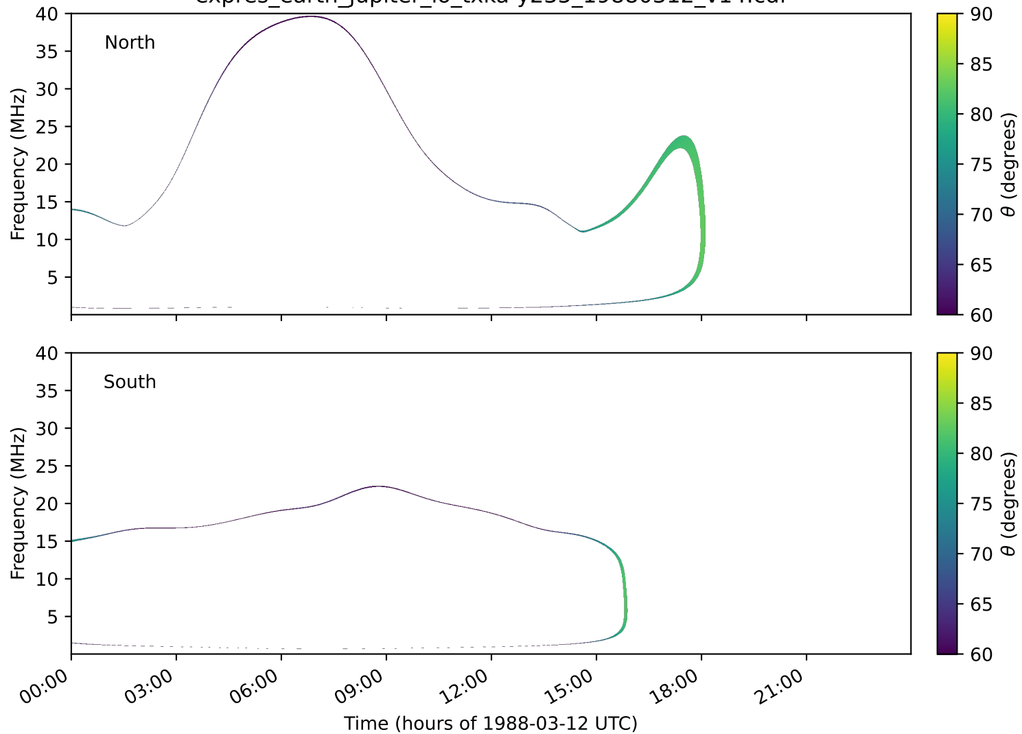
expres_earth_jupiter_io_txka-y235_19880312_v14.cdf
