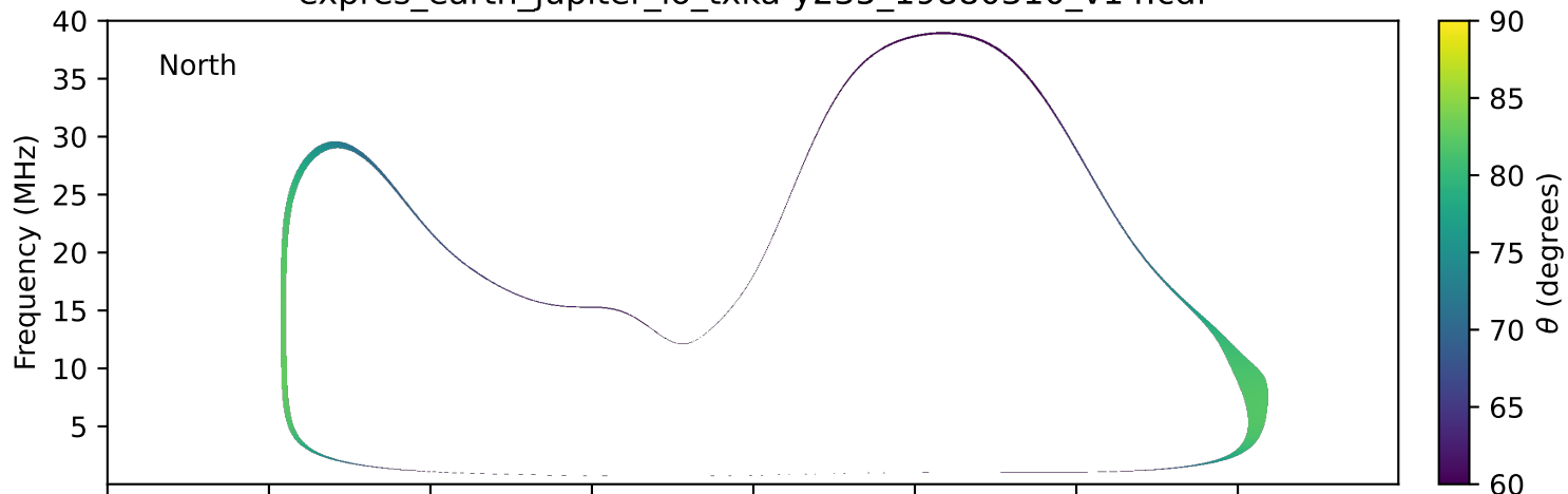
expres_earth_jupiter_io_txka-y235_19880310_v14.cdf
