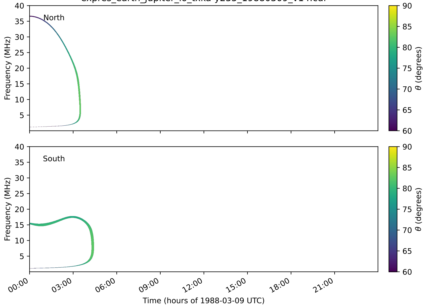
expres_earth_jupiter_io_txka-y235_19880309_v14.cdf
