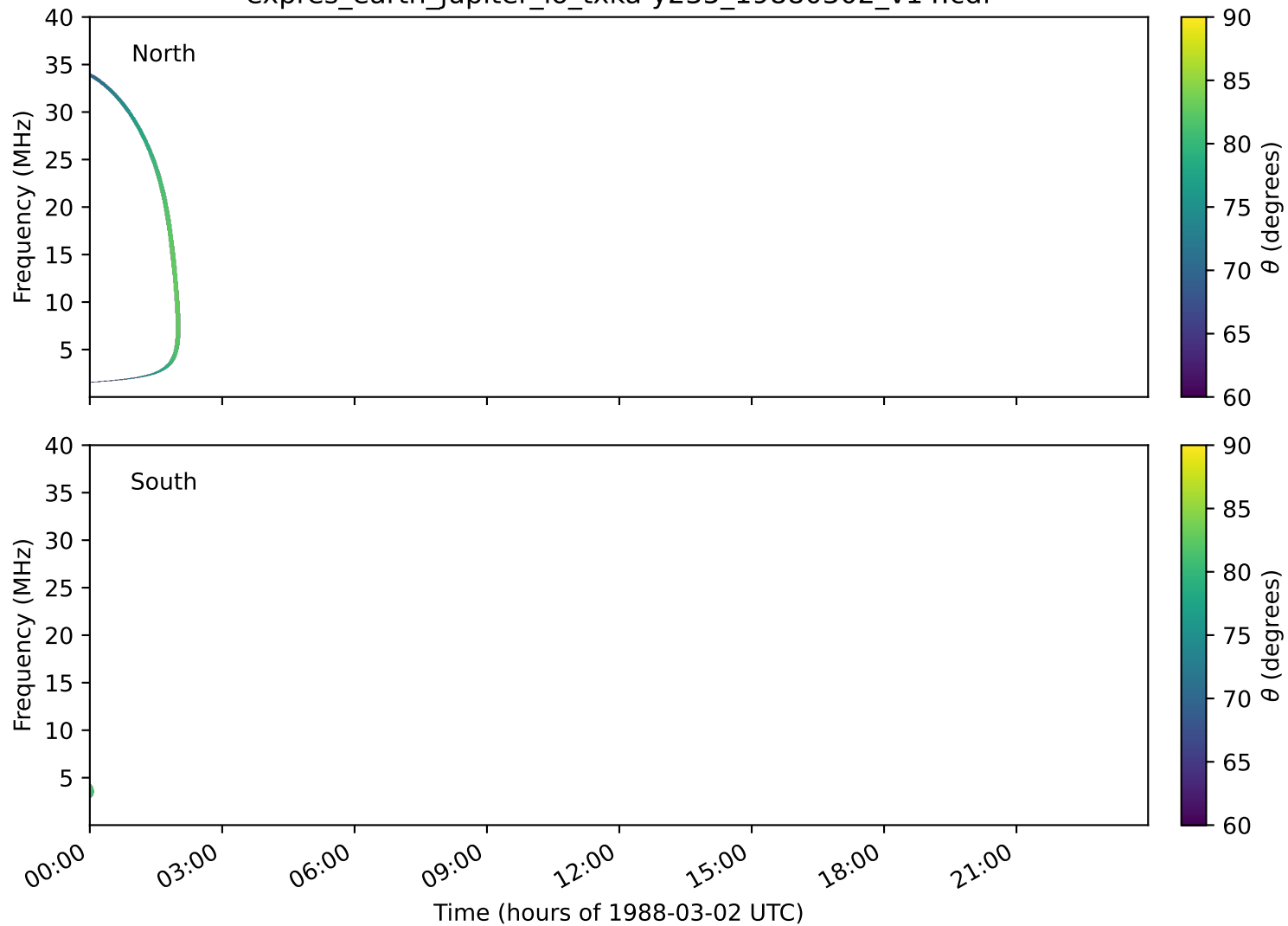
expres_earth_jupiter_io_txka-y235_19880302_v14.cdf
