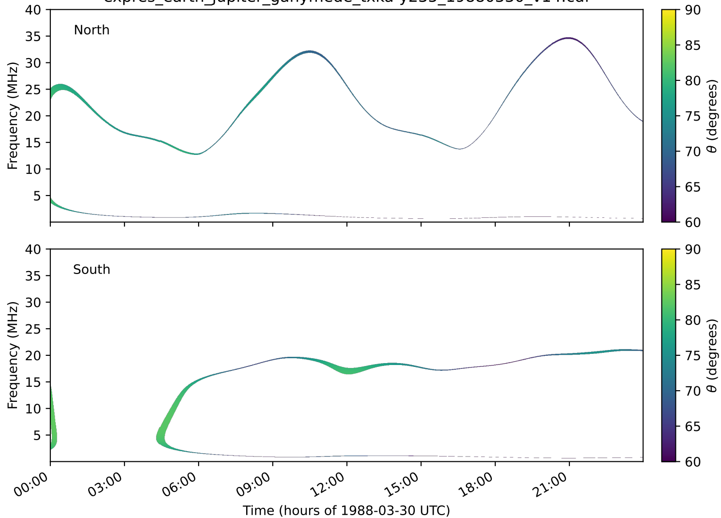
expres_earth_jupiter_ganymede_txka-y235_19880330_v14.cdf
