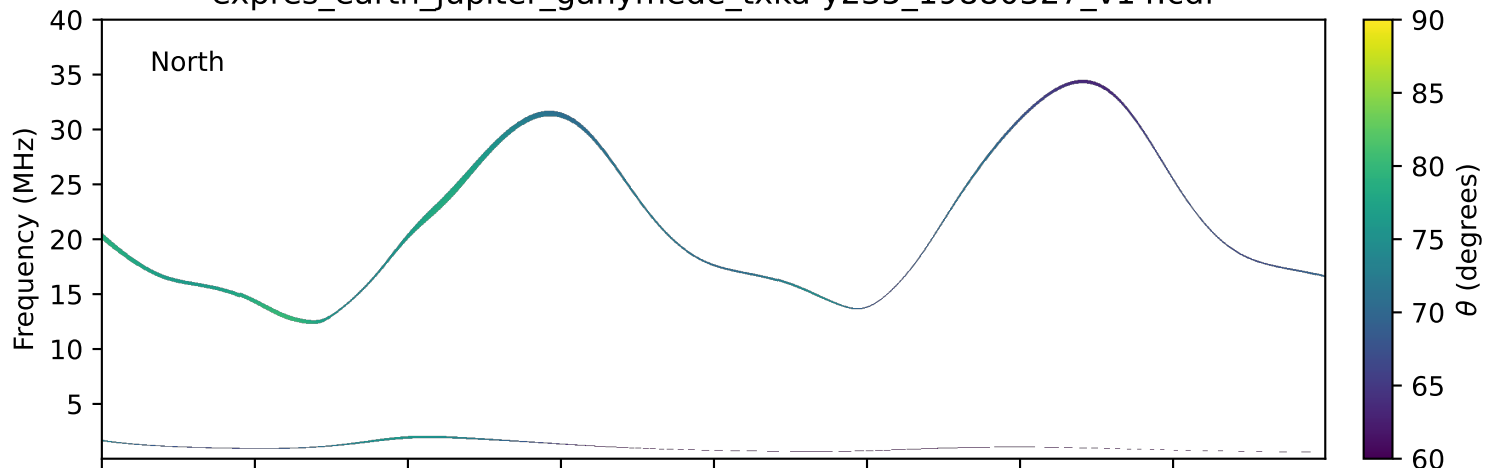
expres_earth_jupiter_ganymede_txka-y235_19880327_v14.cdf
