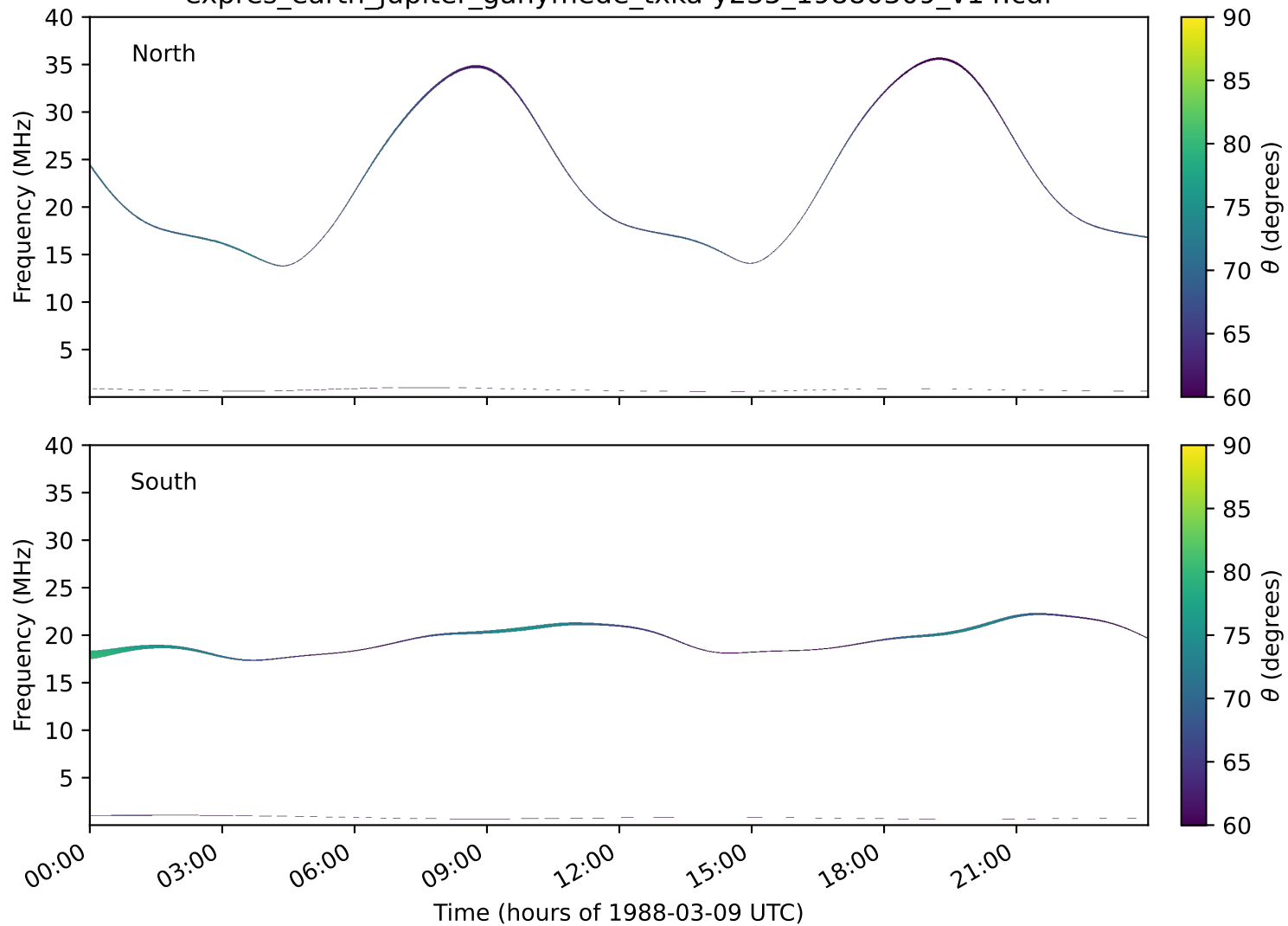
expres_earth_jupiter_ganymede_txka-y235_19880309_v14.cdf
