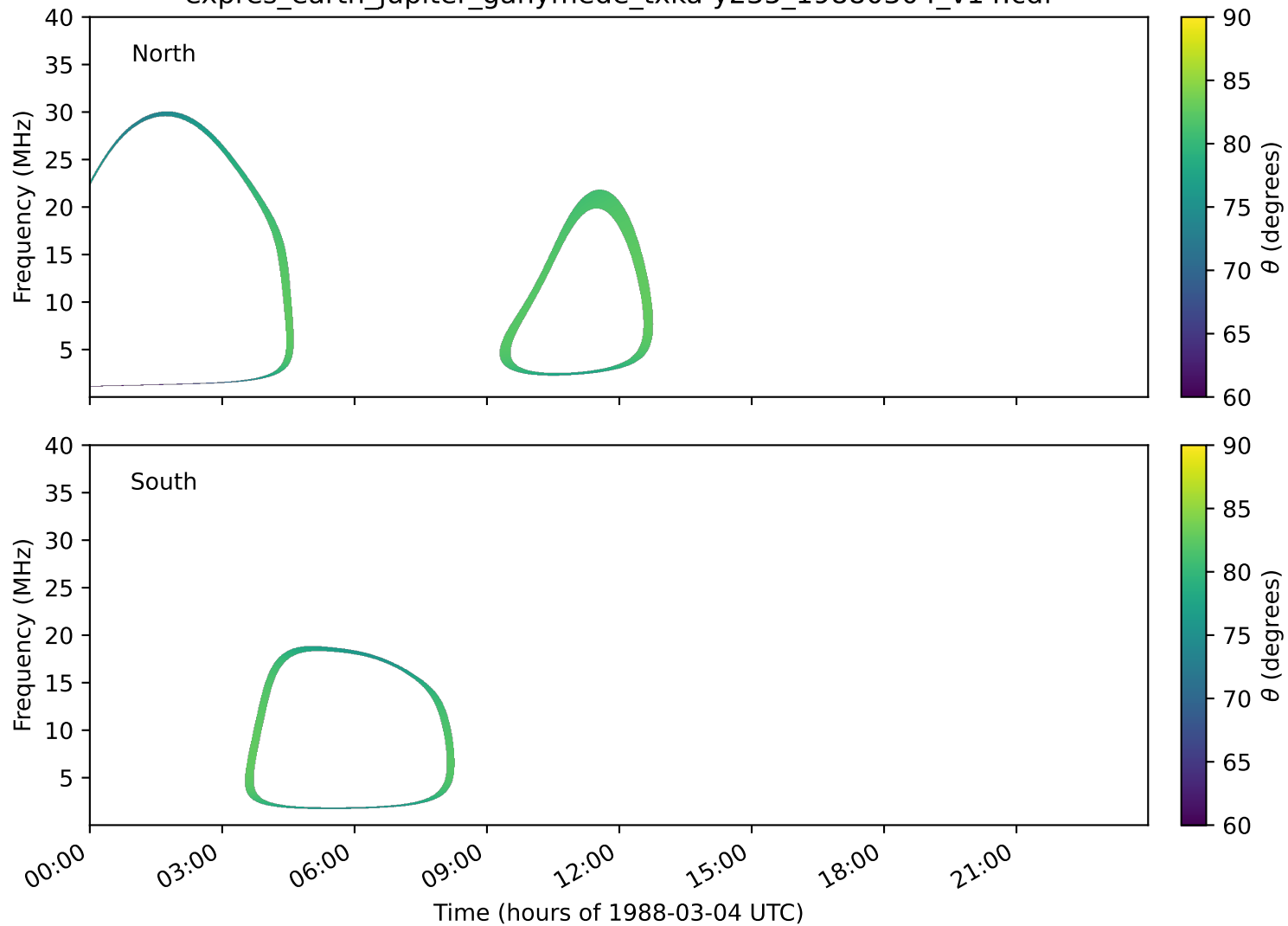
expres_earth_jupiter_ganymede_txka-y235_19880304_v14.cdf
