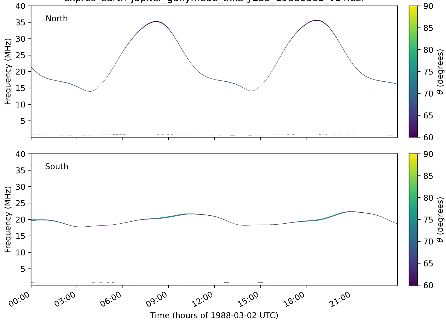
expres_earth_jupiter_ganymede_txka-y235_19880302_v14.cdf
