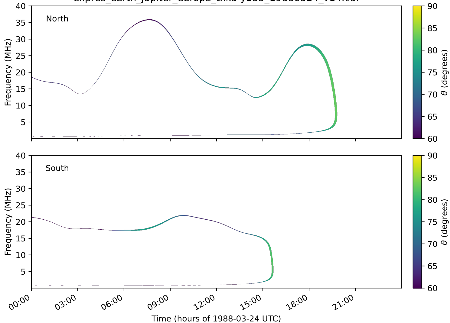
expres_earth_jupiter_europa_txka-y235_19880324_v14.cdf
