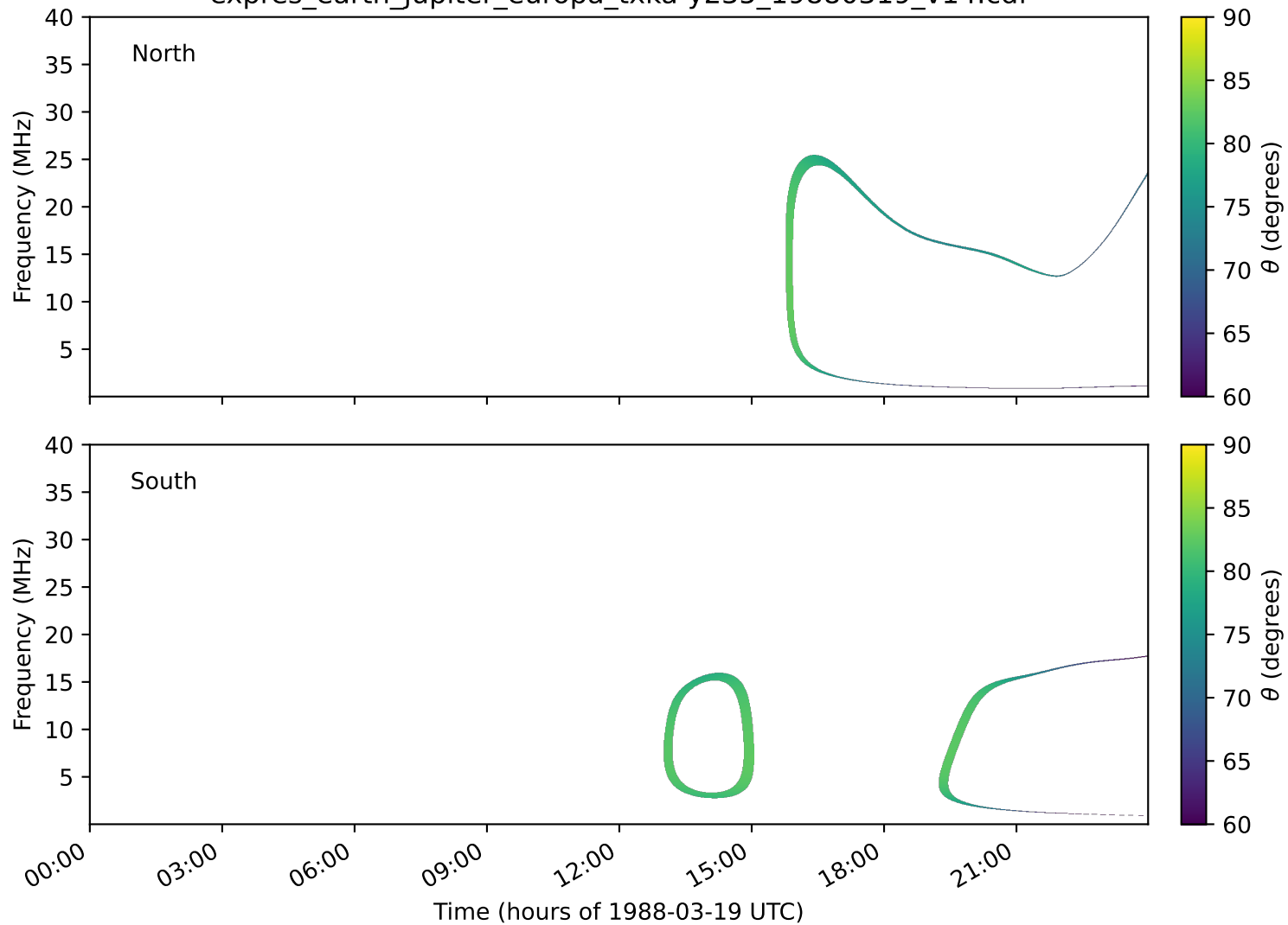
expres_earth_jupiter_europa_txka-y235_19880319_v14.cdf
