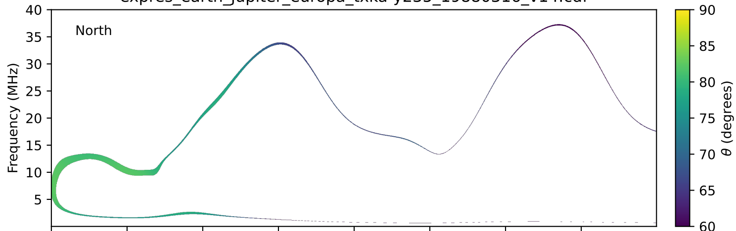
expres_earth_jupiter_europa_txka-y235_19880316_v14.cdf
