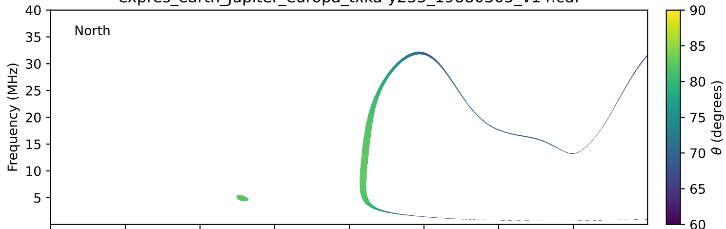
expres_earth_jupiter_europa_txka-y235_19880305_v14.cdf
