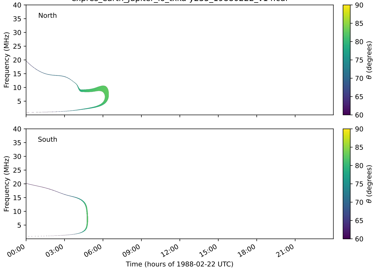
expres_earth_jupiter_io_txka-y235_19880222_v14.cdf
