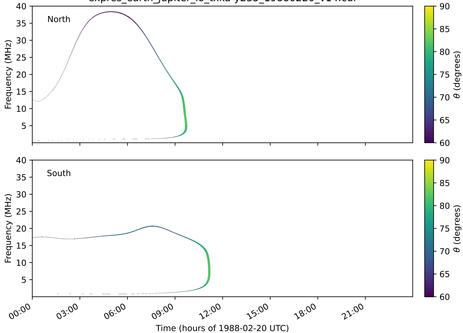
expres_earth_jupiter_io_txka-y235_19880220_v14.cdf
