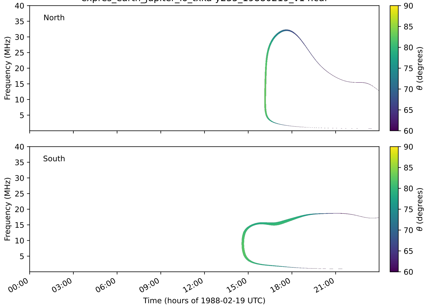
expres_earth_jupiter_io_txka-y235_19880219_v14.cdf
