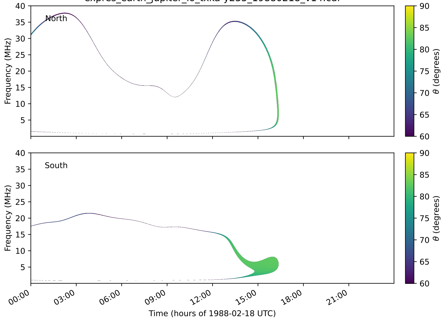
expres_earth_jupiter_io_txka-y235_19880218_v14.cdf
