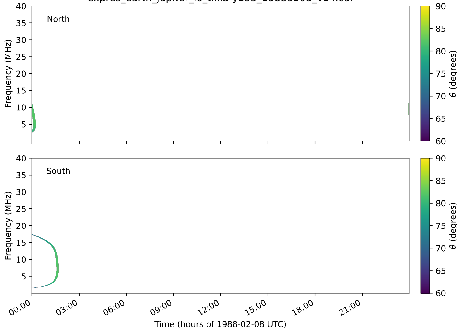
expres_earth_jupiter_io_txka-y235_19880208_v14.cdf
