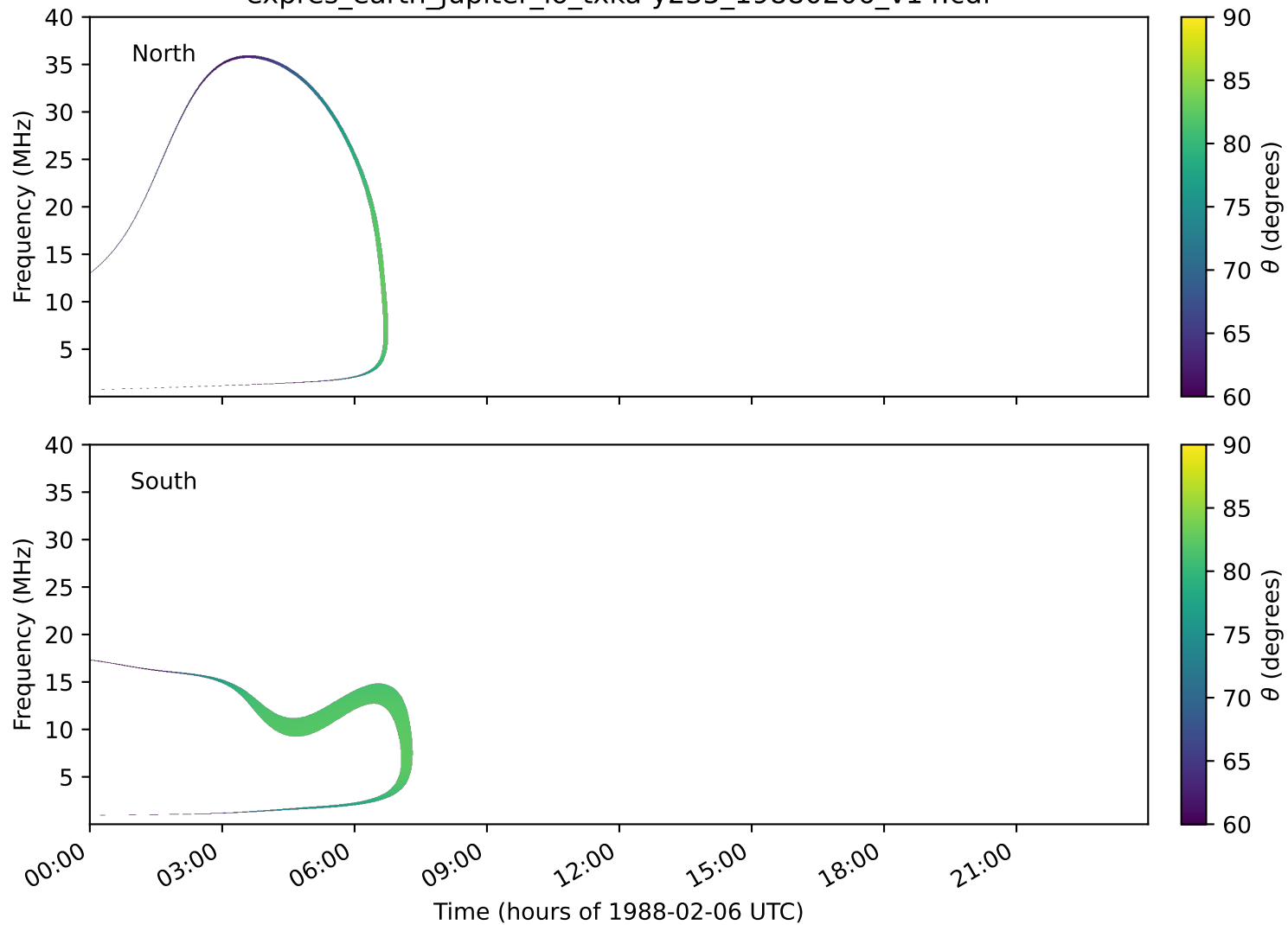
expres_earth_jupiter_io_txka-y235_19880206_v14.cdf
