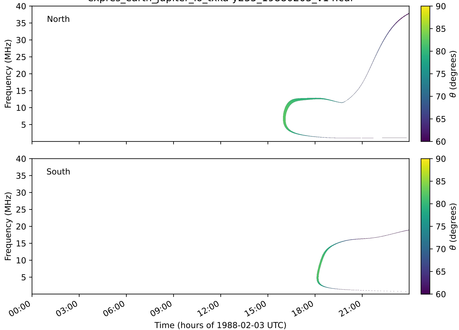
expres_earth_jupiter_io_txka-y235_19880203_v14.cdf
