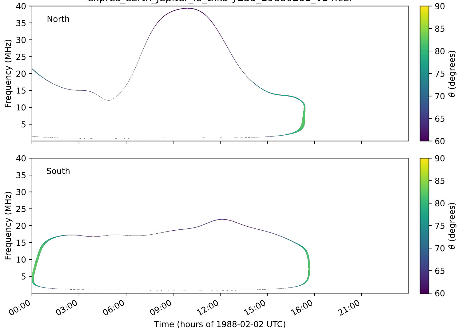
expres_earth_jupiter_io_txka-y235_19880202_v14.cdf
