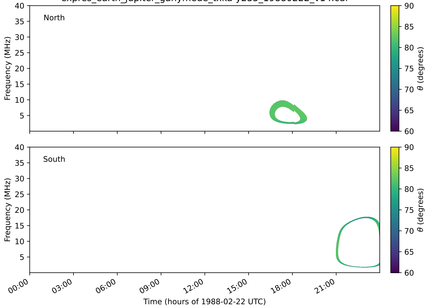
expres_earth_jupiter_ganymede_txka-y235_19880222_v14.cdf
