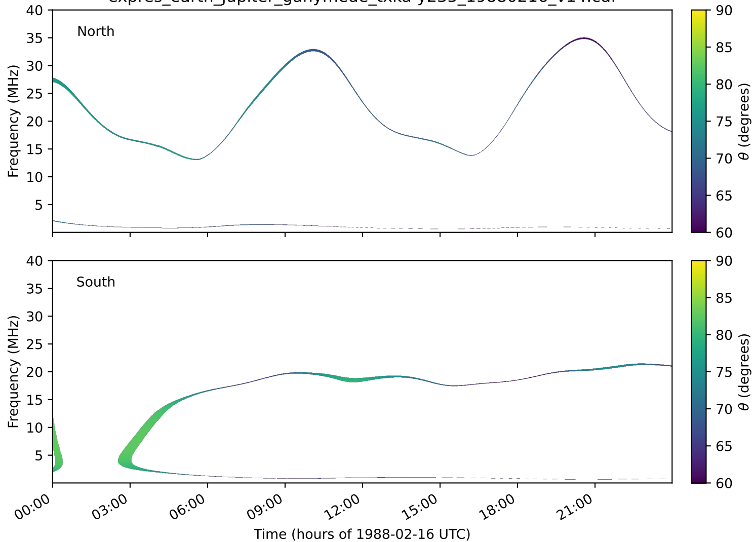
expres_earth_jupiter_ganymede_txka-y235_19880216_v14.cdf
