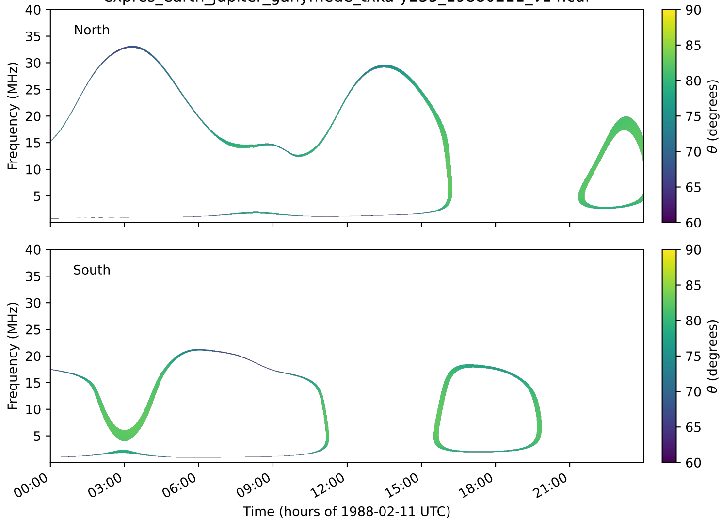
expres_earth_jupiter_ganymede_txka-y235_19880211_v14.cdf
