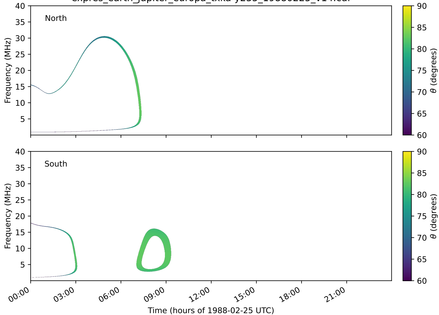
expres_earth_jupiter_europa_txka-y235_19880225_v14.cdf
