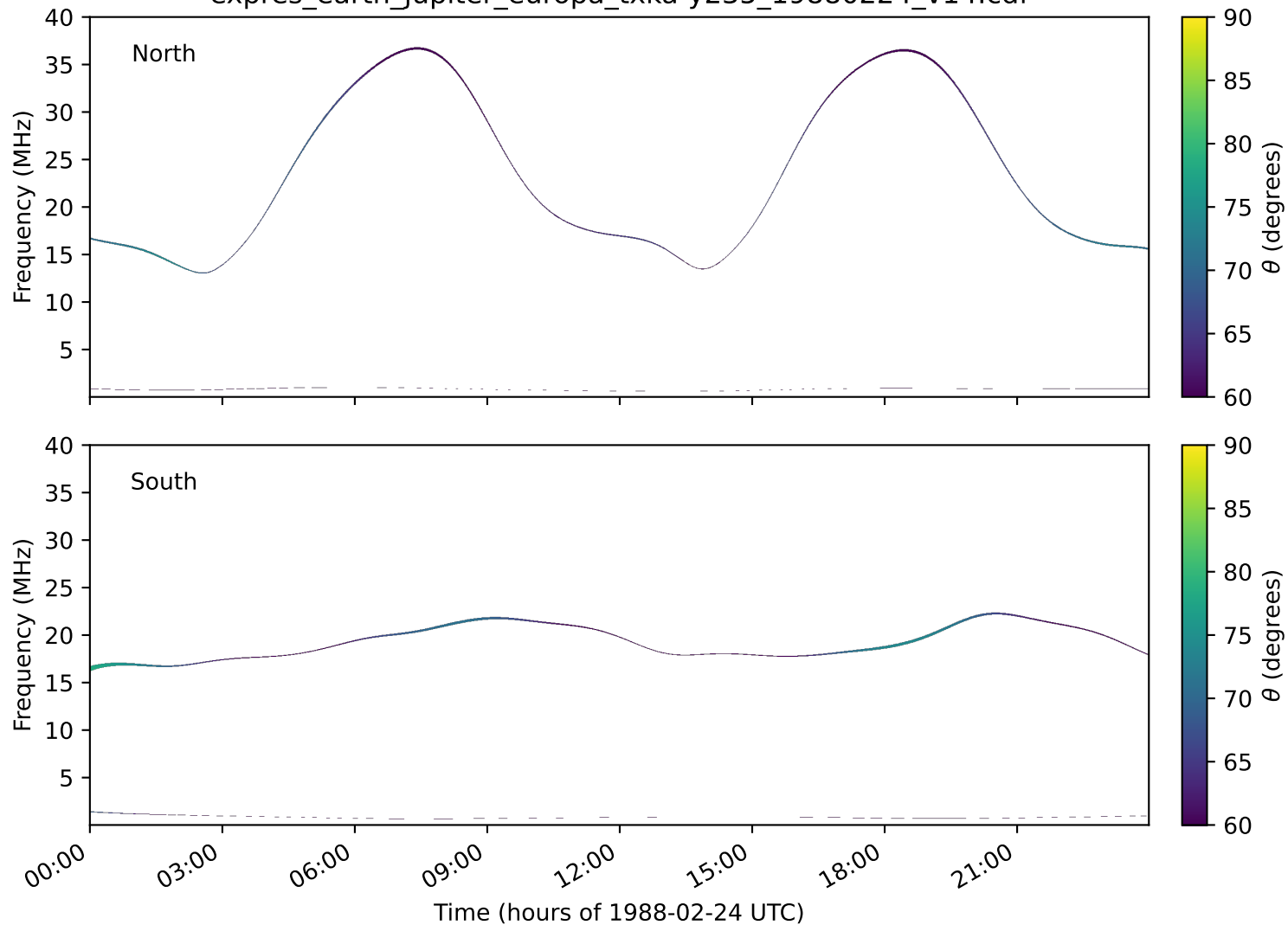
expres_earth_jupiter_europa_txka-y235_19880224_v14.cdf
