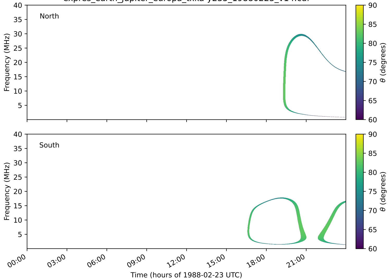
expres_earth_jupiter_europa_txka-y235_19880223_v14.cdf
