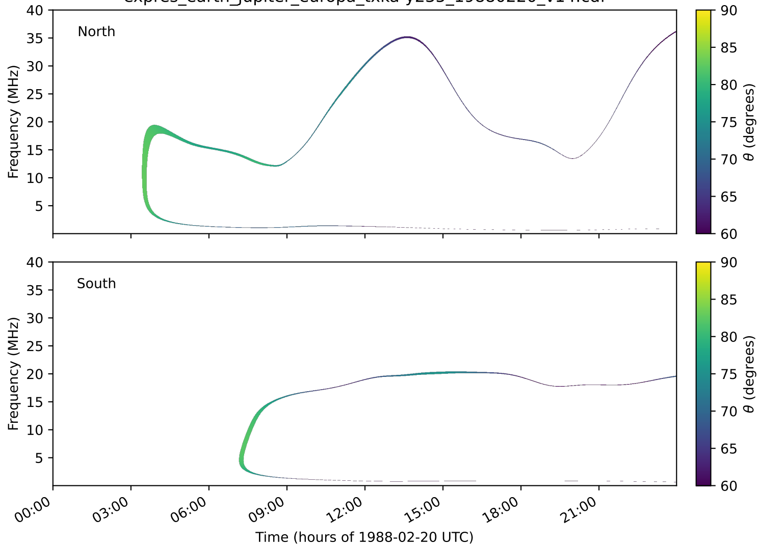
expres_earth_jupiter_europa_txka-y235_19880220_v14.cdf
