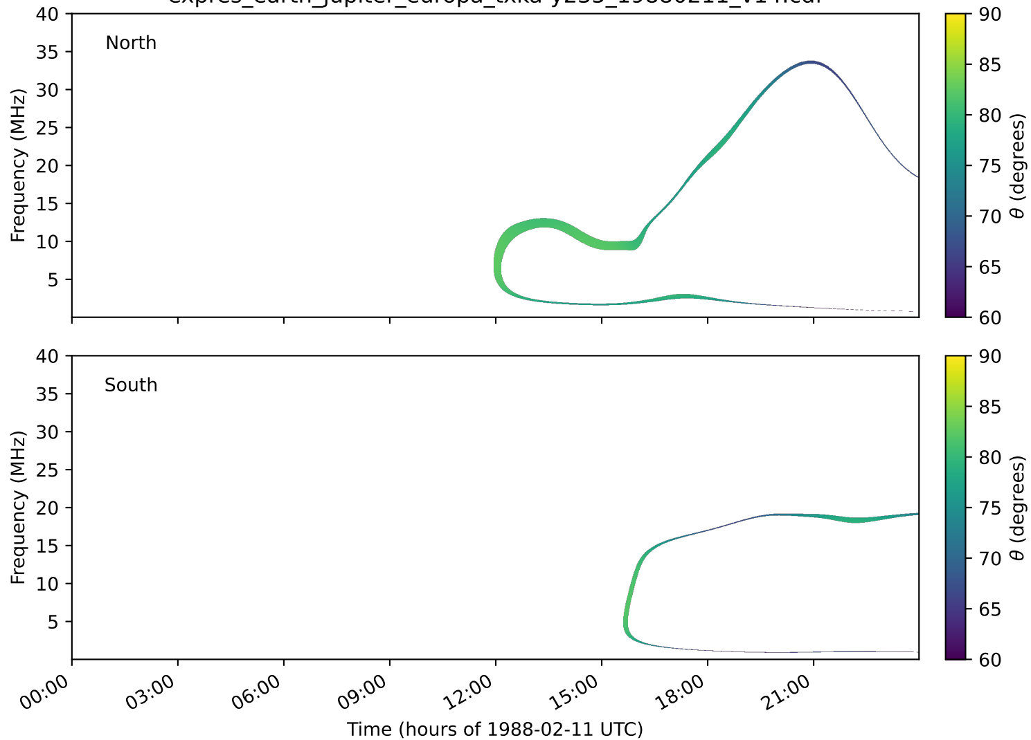
expres_earth_jupiter_europa_txka-y235_19880211_v14.cdf
