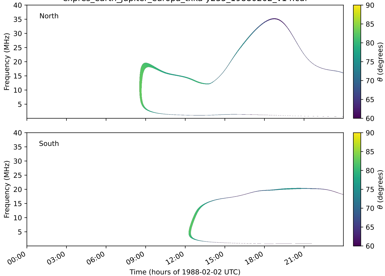
expres_earth_jupiter_europa_txka-y235_19880202_v14.cdf
