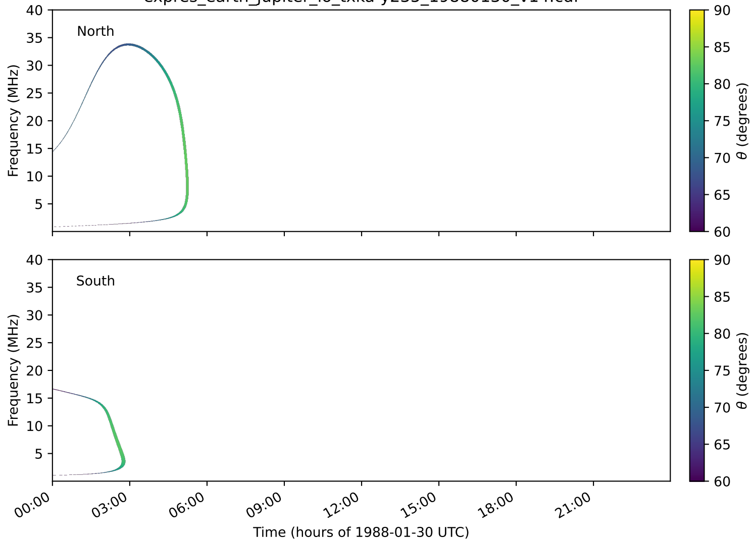
expres_earth_jupiter_io_txka-y235_19880130_v14.cdf
