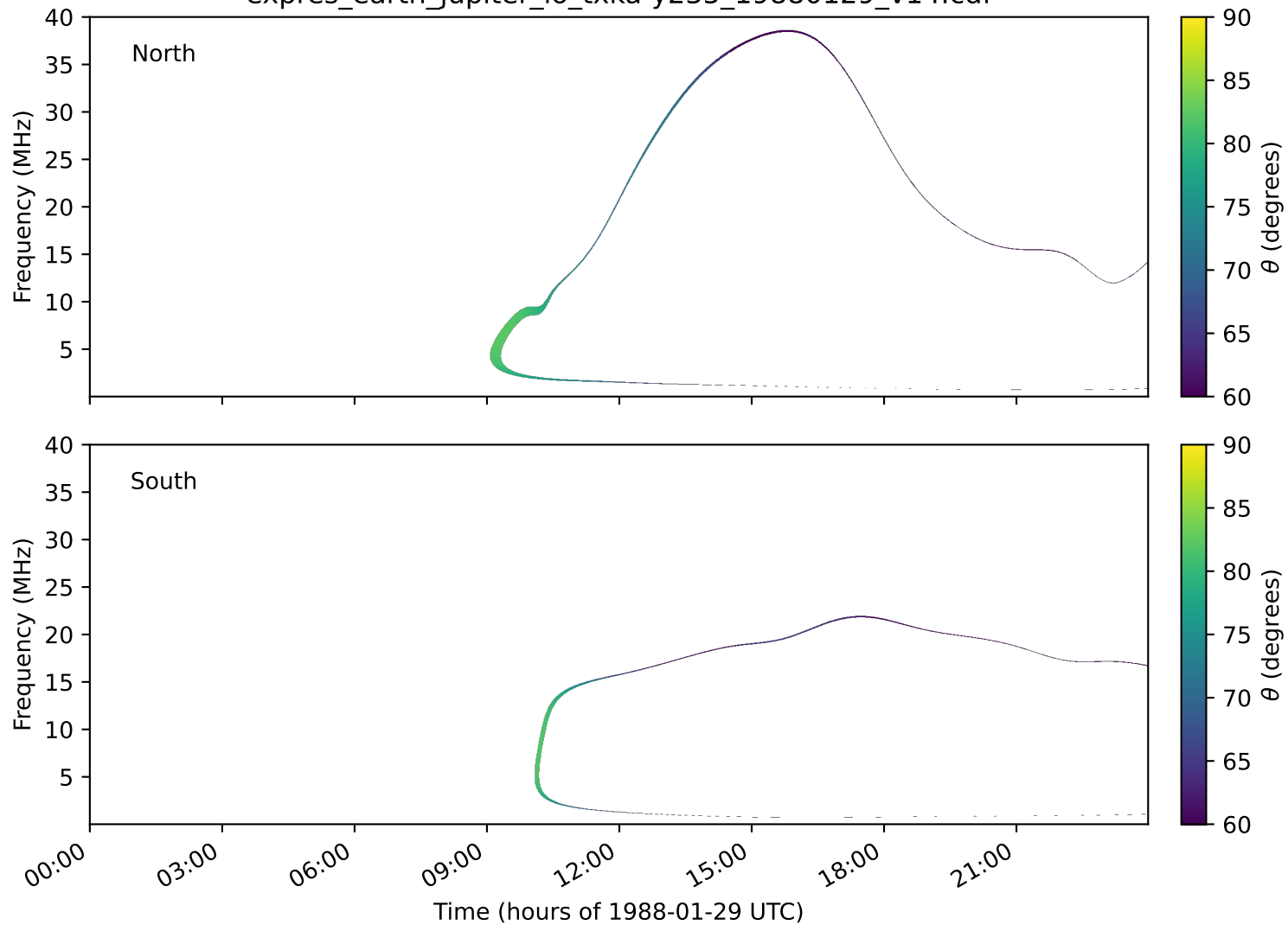
expres_earth_jupiter_io_txka-y235_19880129_v14.cdf
