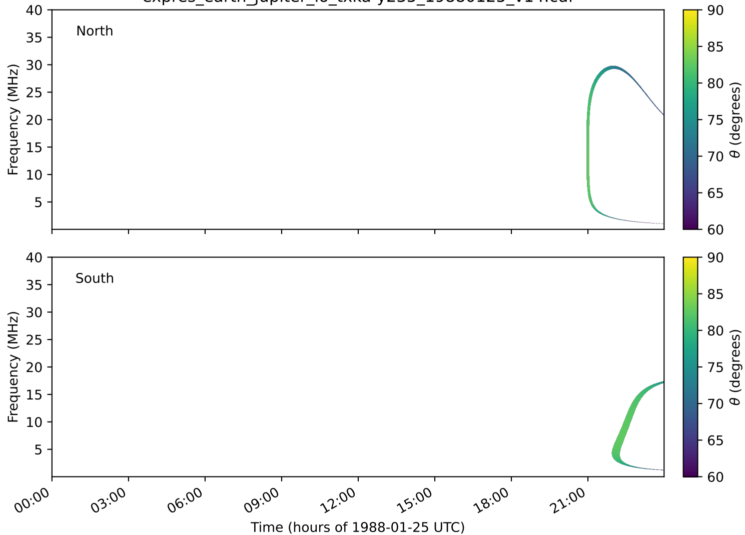
expres_earth_jupiter_io_txka-y235_19880125_v14.cdf
