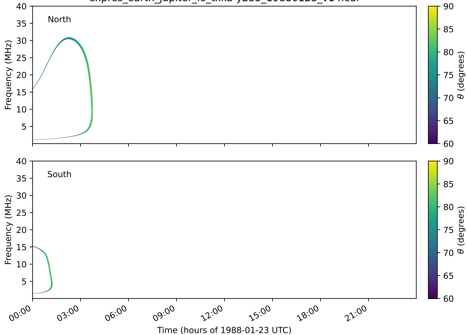
expres_earth_jupiter_io_txka-y235_19880123_v14.cdf
