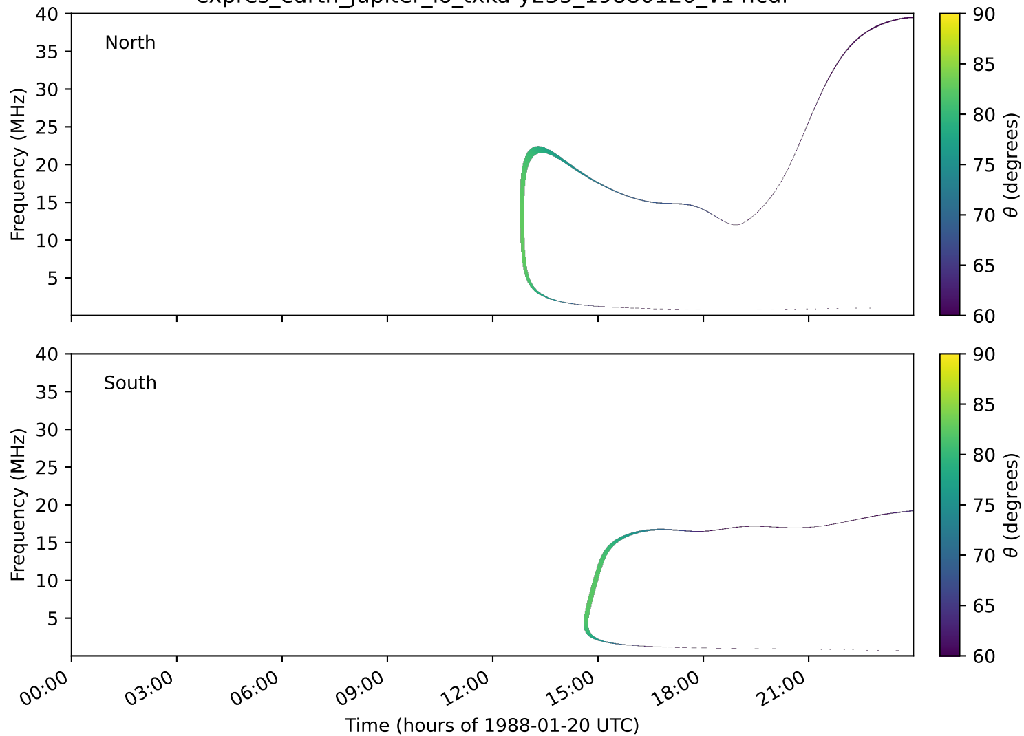
expres_earth_jupiter_io_txka-y235_19880120_v14.cdf
