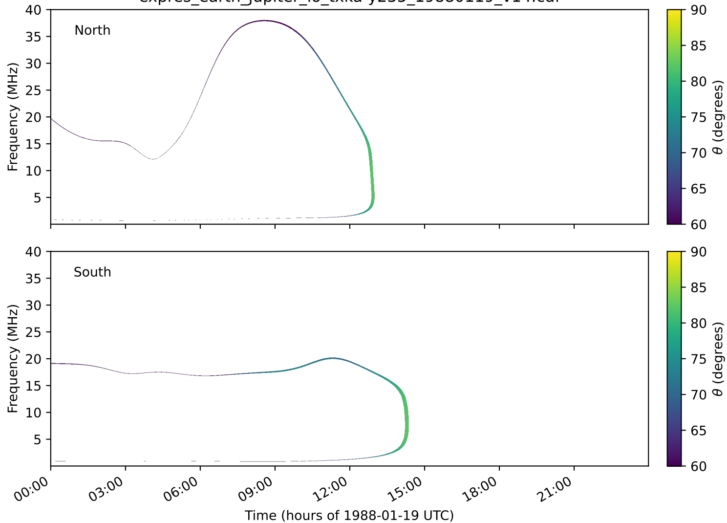
expres_earth_jupiter_io_txka-y235_19880119_v14.cdf
