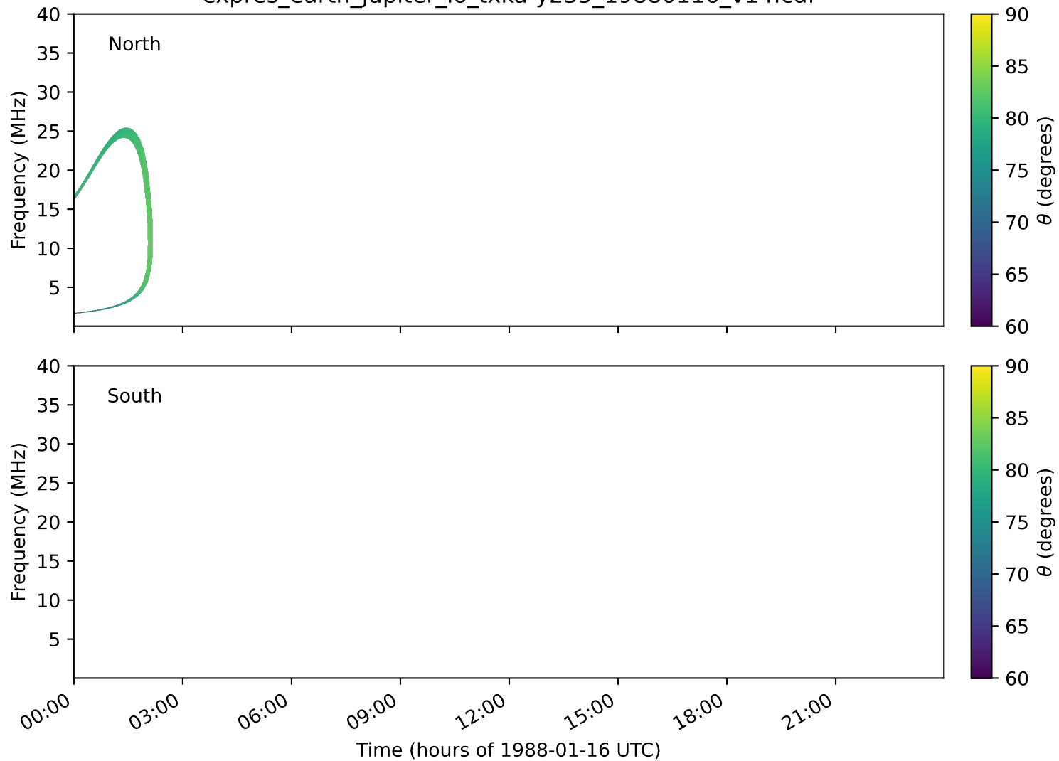
expres_earth_jupiter_io_txka-y235_19880116_v14.cdf
