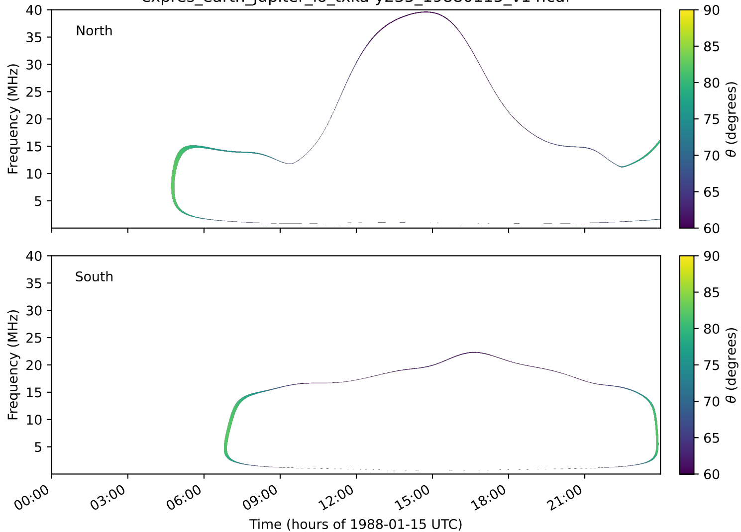
expres_earth_jupiter_io_txka-y235_19880115_v14.cdf
