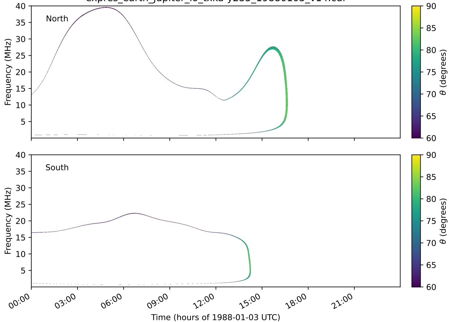
expres_earth_jupiter_io_txka-y235_19880103_v14.cdf
