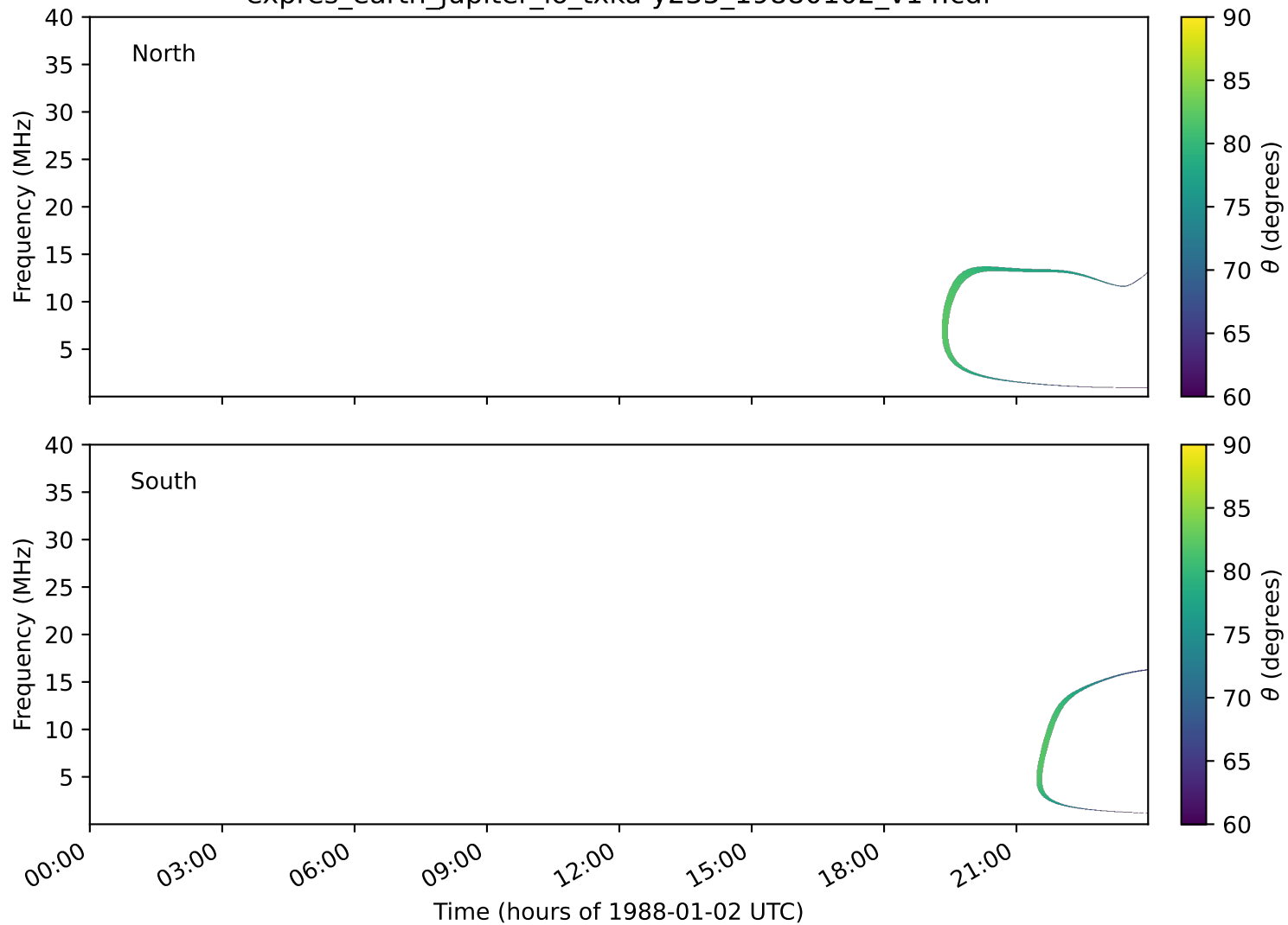
expres_earth_jupiter_io_txka-y235_19880102_v14.cdf
