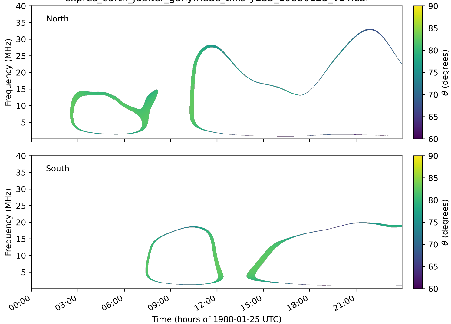
expres_earth_jupiter_ganymede_txka-y235_19880125_v14.cdf
