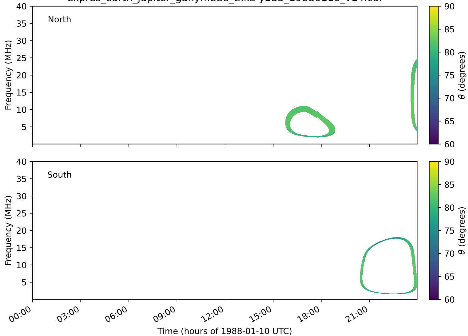
expres_earth_jupiter_ganymede_txka-y235_19880110_v14.cdf
