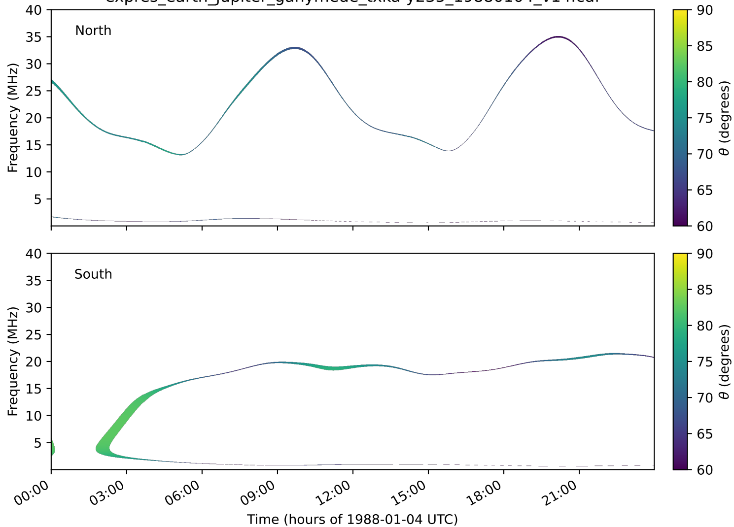
expres_earth_jupiter_ganymede_txka-y235_19880104_v14.cdf
