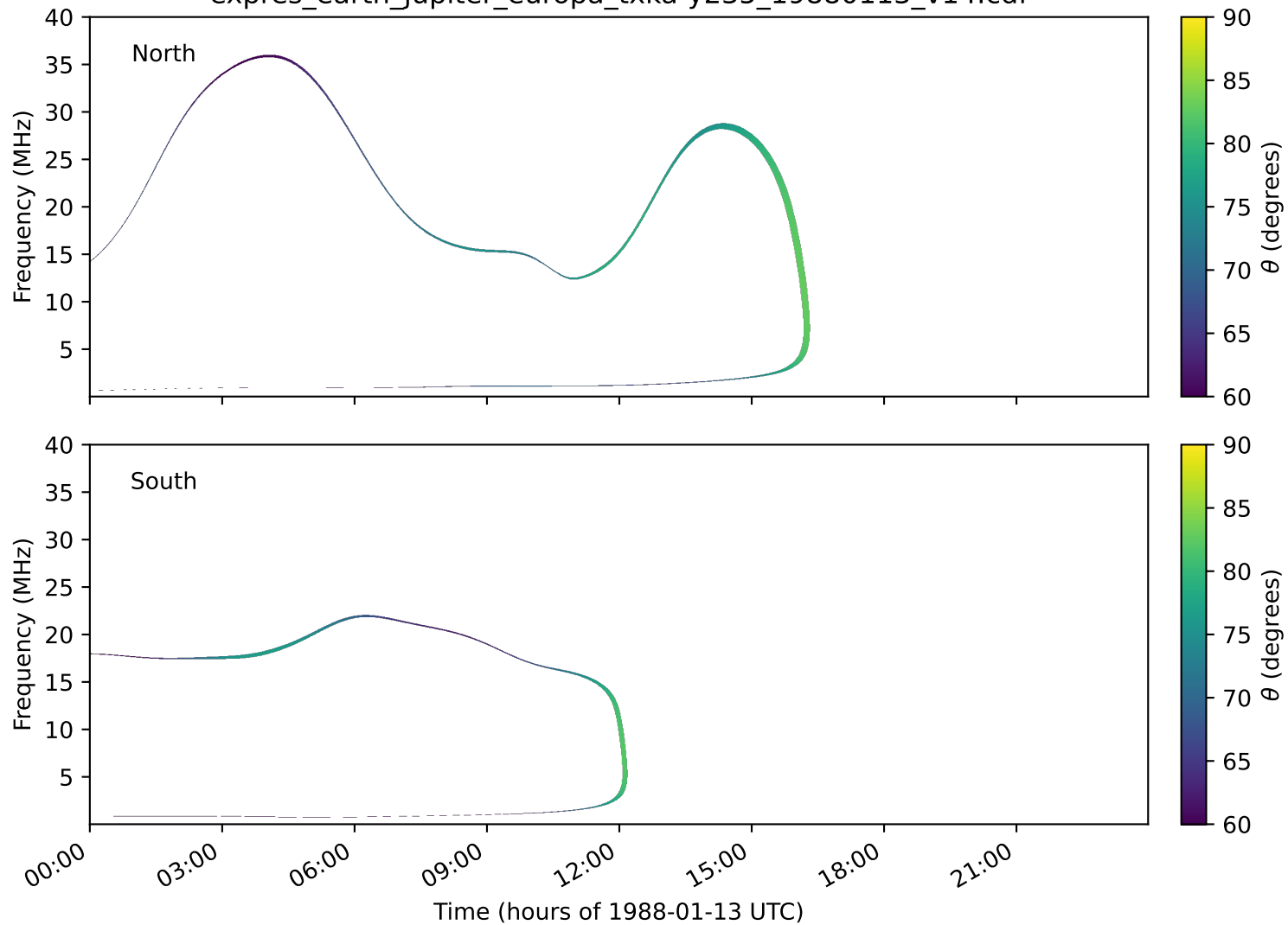
expres_earth_jupiter_europa_txka-y235_19880113_v14.cdf
