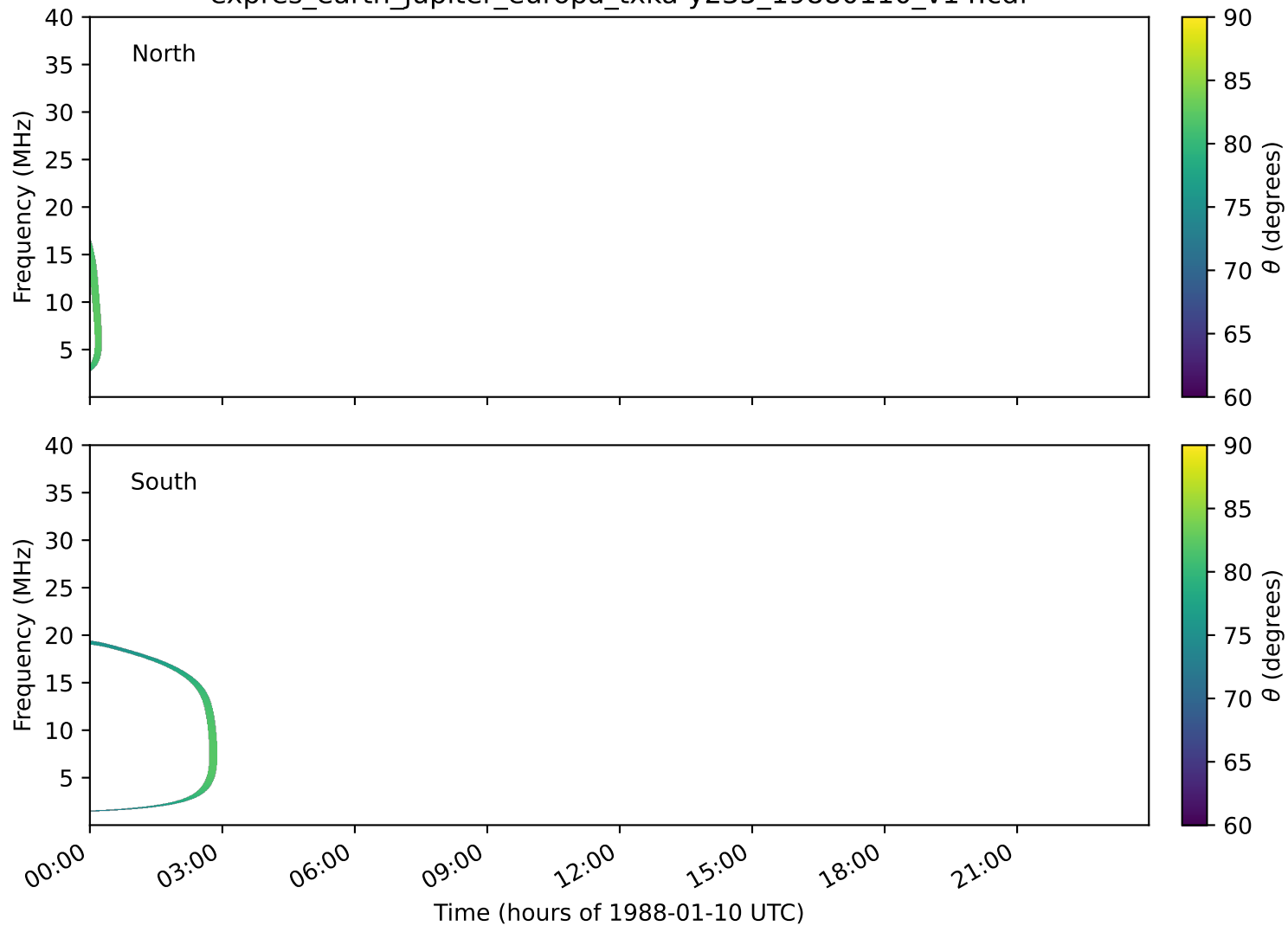
expres_earth_jupiter_europa_txka-y235_19880110_v14.cdf
