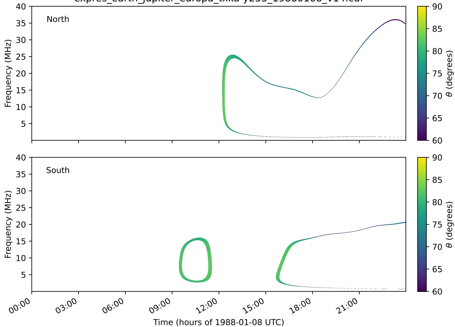
expres_earth_jupiter_europa_txka-y235_19880108_v14.cdf
