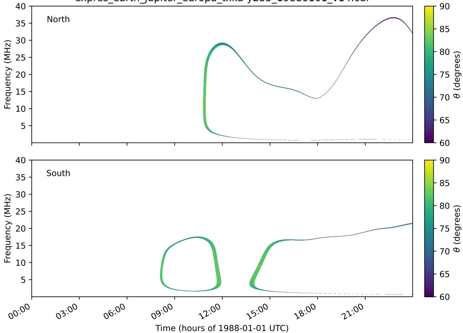
expres_earth_jupiter_europa_txka-y235_19880101_v14.cdf
