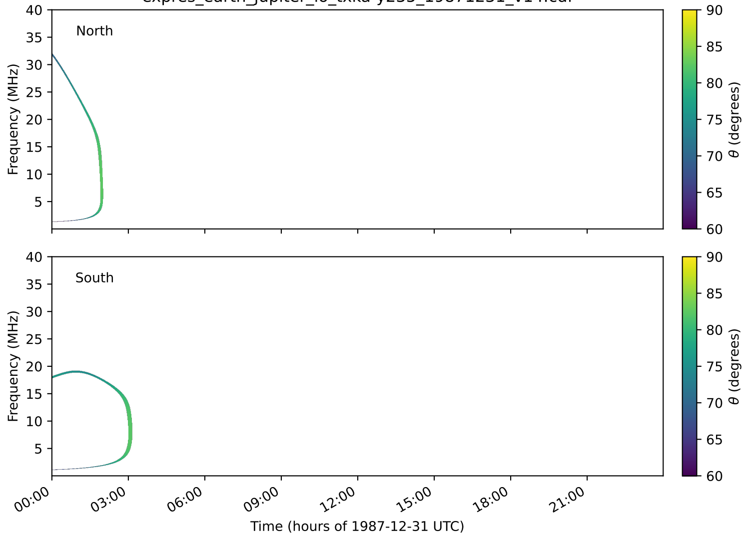
expres_earth_jupiter_io_txka-y235_19871231_v14.cdf
